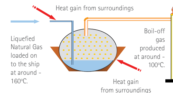
Figure 3. Schematic showing how JBOG Recovery works
