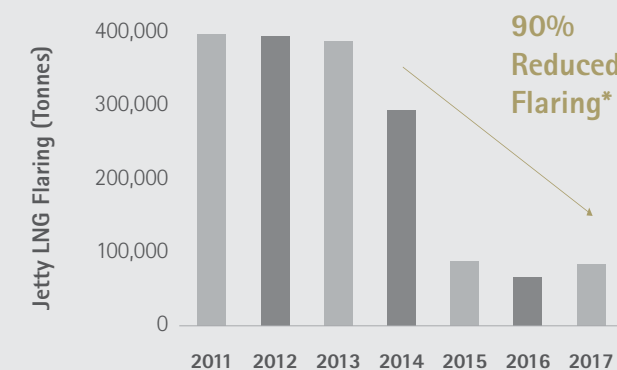
Figure 2. Reduction in JBOG Flaring 2011-2017 *
