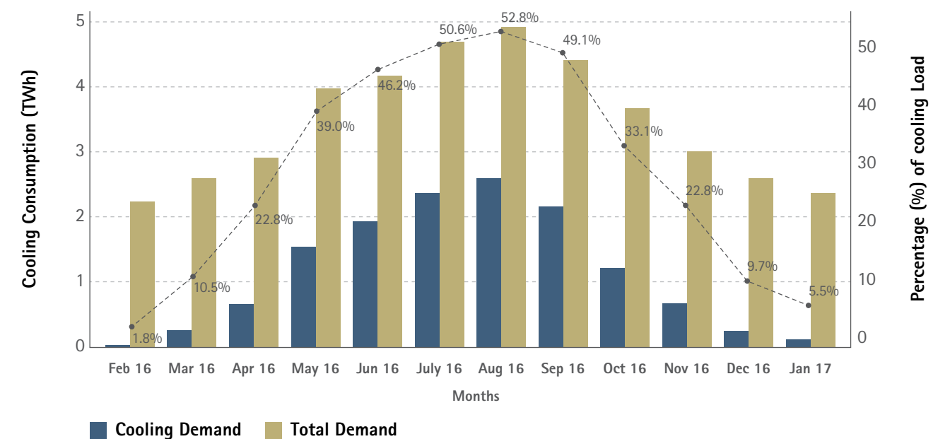
Figure 1: Electricity and cooling demand
