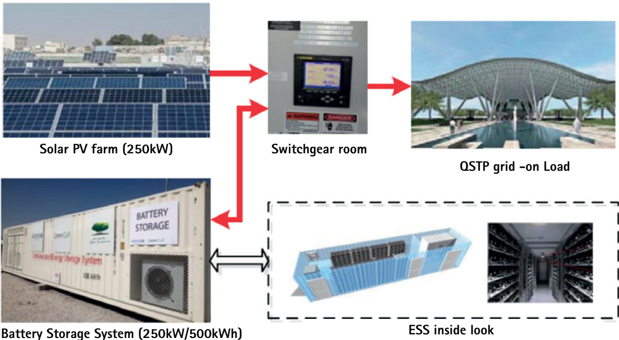
generation/storage micro-grid system, shown in Fig. 10, has been installed in the Solar Test Facility (STF) near Doha, Qatar. Figure 10. Overview of the hybrid solar/Energy Storage System micro-grid
