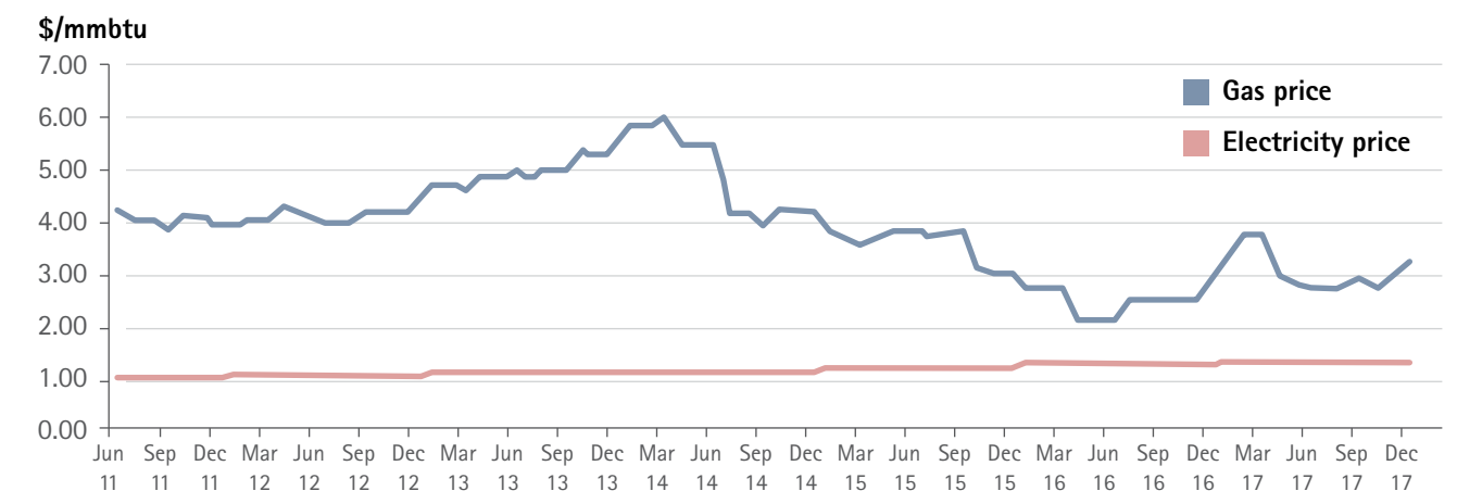
Fig 1. Market price for gas vs the price of gas for electricity
