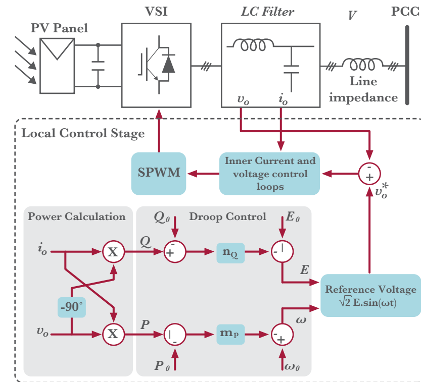
Figure 4. The simplified control scheme of traditional droop control for DG [7]
